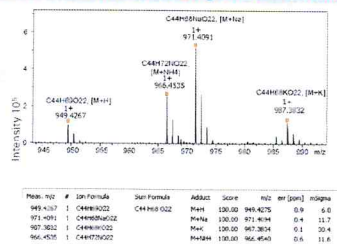
Nicotianoside II and adduct assignments from SmartFormula.
